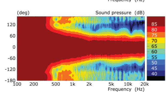
Blade One Meta Spinorama (top) and dispersion plots - horizontal (middle) and vertical (bottom)
