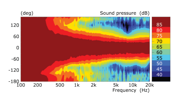
Blade Two Meta Spinorama (top) and dispersion plots - horizontal (middle) and vertical (bottom)
