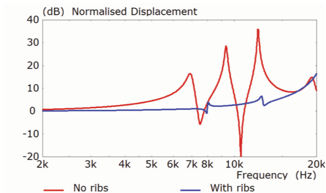
Figure 7. Simulated displacement of tangerine waveguide
